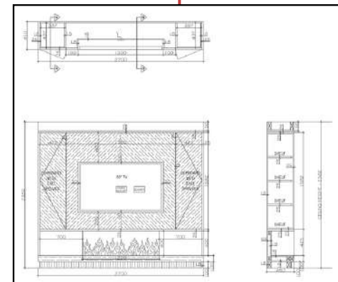
SNUG MEDIA UNIT DESIGN
