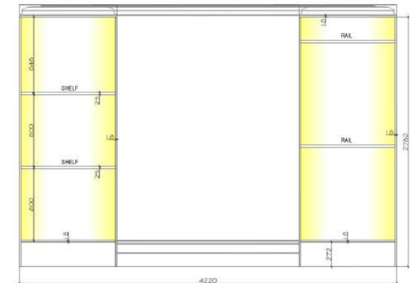
HIDDEN JOINERY
