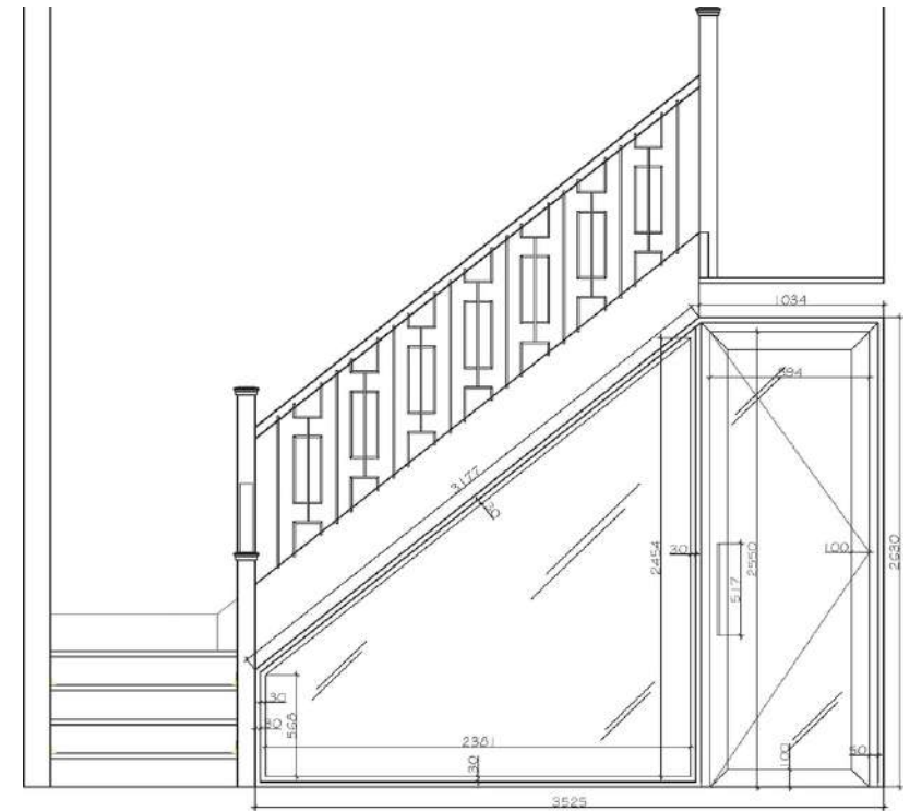
FRONT ELEVATION - GLAZING
