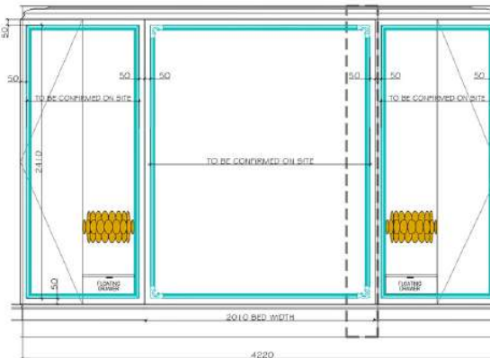
PANELLING & JIB DOOR SETTING OUT
