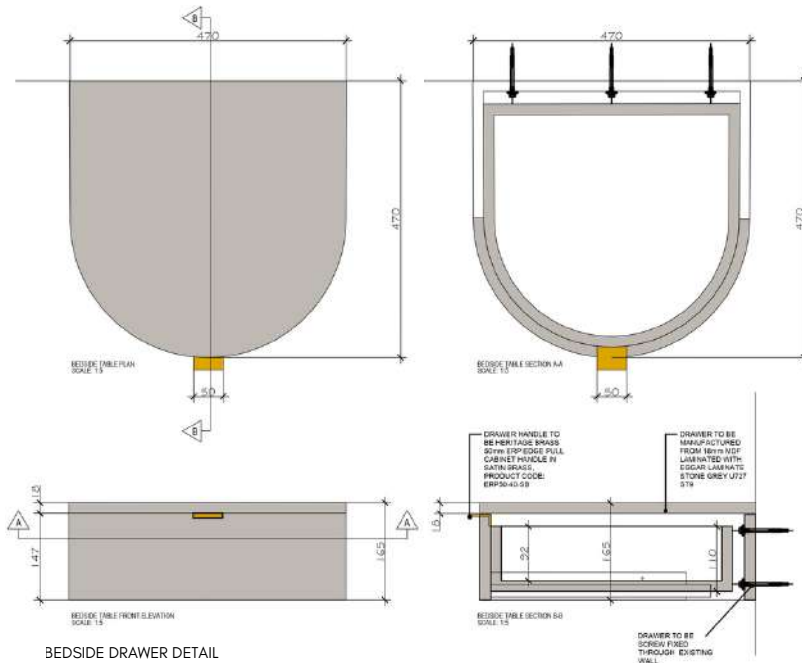
BEDSIDE DRAWER DETAIL
