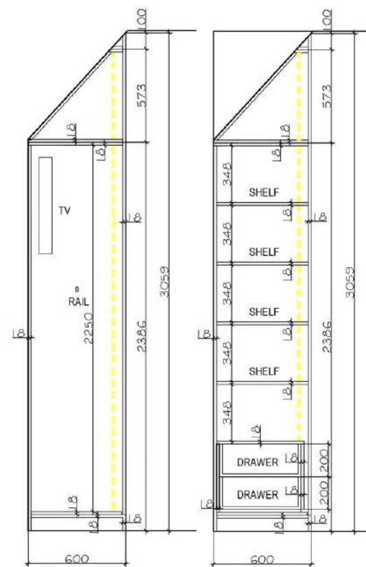
SECTION THROUGH A-A
