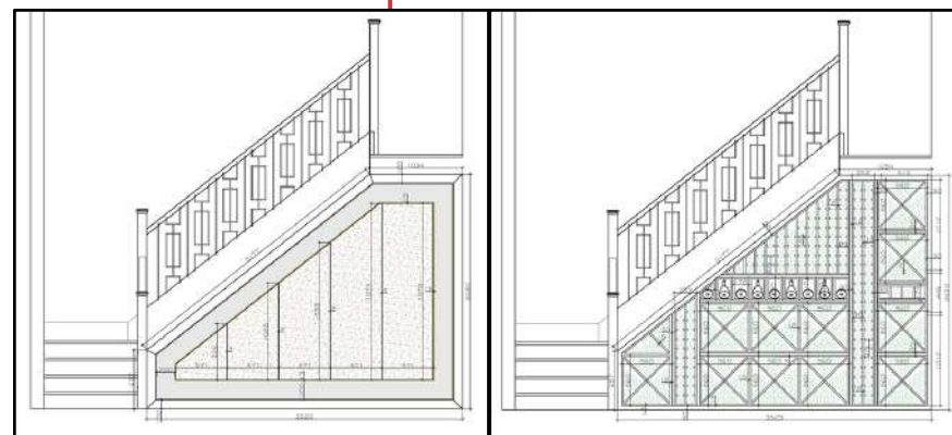
UNDER STAIR JOINERY DESIGN
