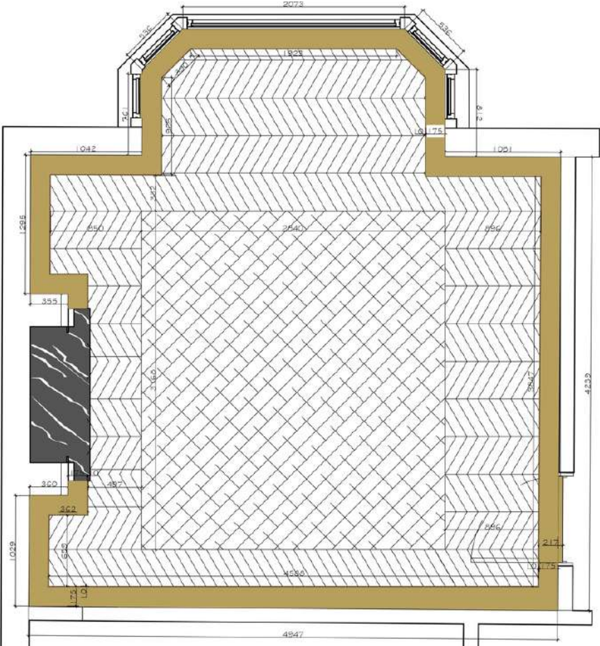
FLOOR FINISHES PLAN
