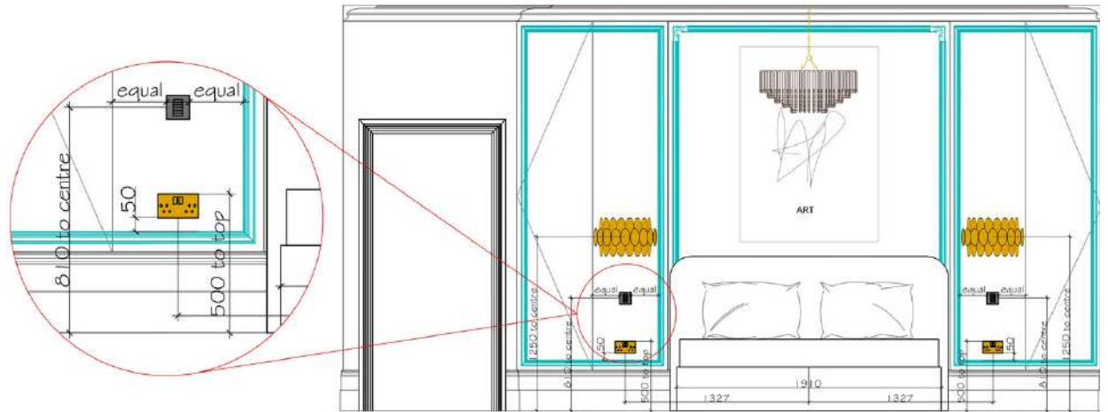
BEDSIDE SOCKET SETTING OUT
