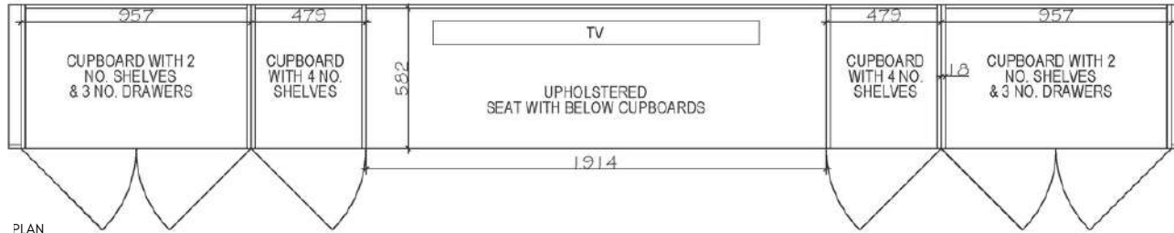
PLAN
