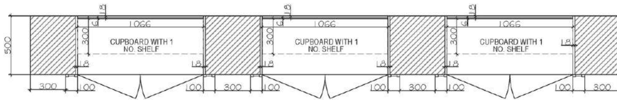
PLAN
