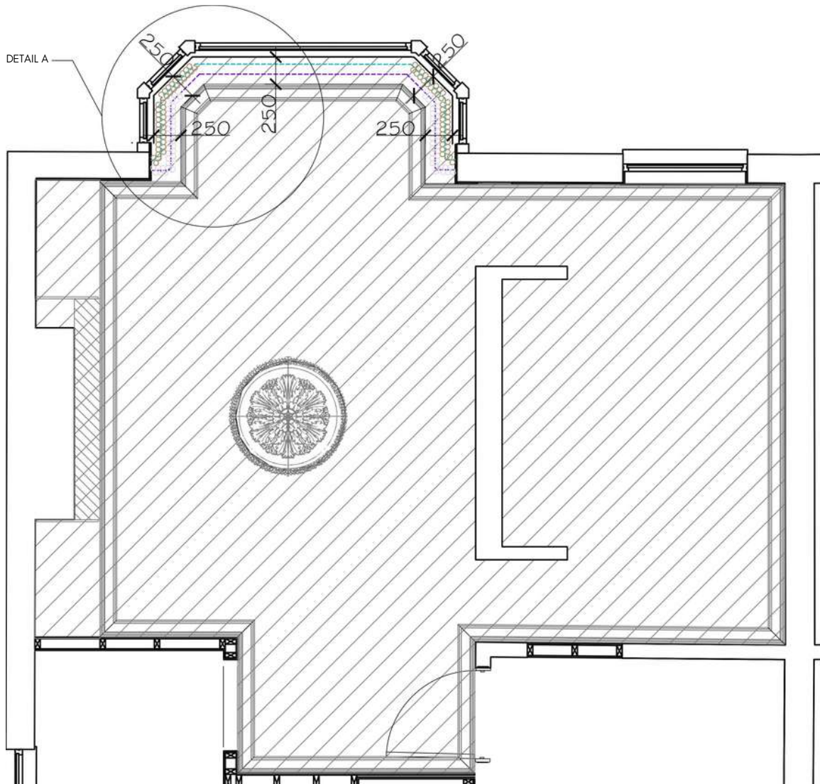
CEILING FINISHES PLAN
