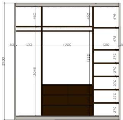
ELEVATION B - INTERNAL
