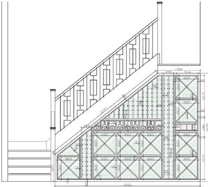
FRONT ELEVATION - WINE STORAGE JOINERY
