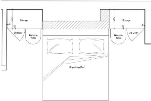
PLAN OF BED & HIDDEN JOINERY
