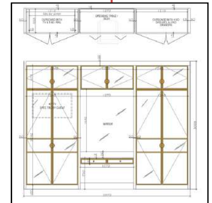
GUEST BEDROOM WARDROBE
