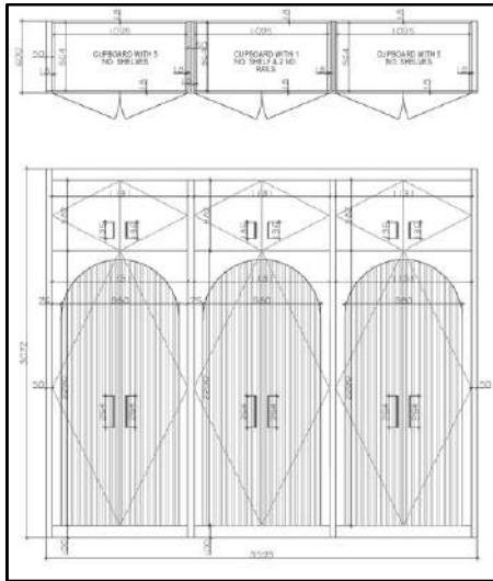
CHILD'S BEDROOM WARDROBE
