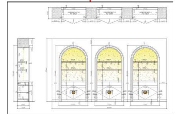
ENTERTAINMENT ROOM JOINERY
