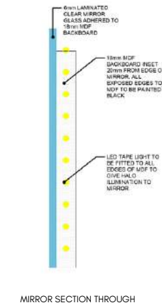
MIRROR SECTION THROUGH
