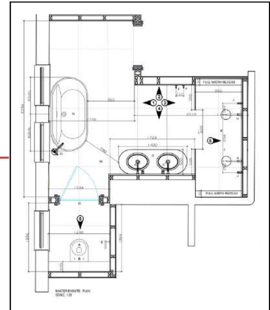
BATHROOM DESIGN
