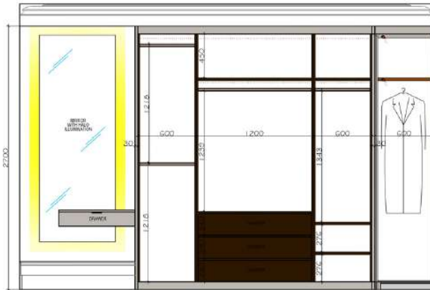
ELEVATION A - INTERNAL
