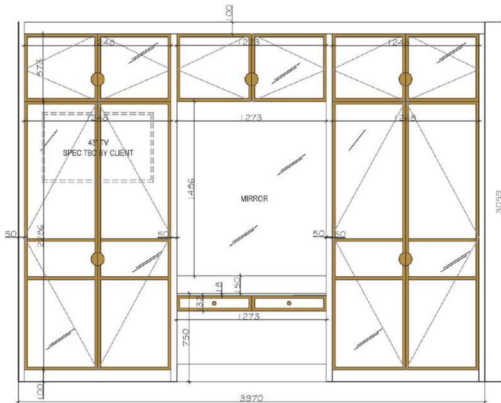
FRONT ELEVATION
