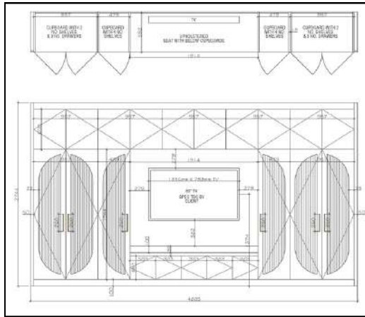
PLAY ROOM JOINERY
